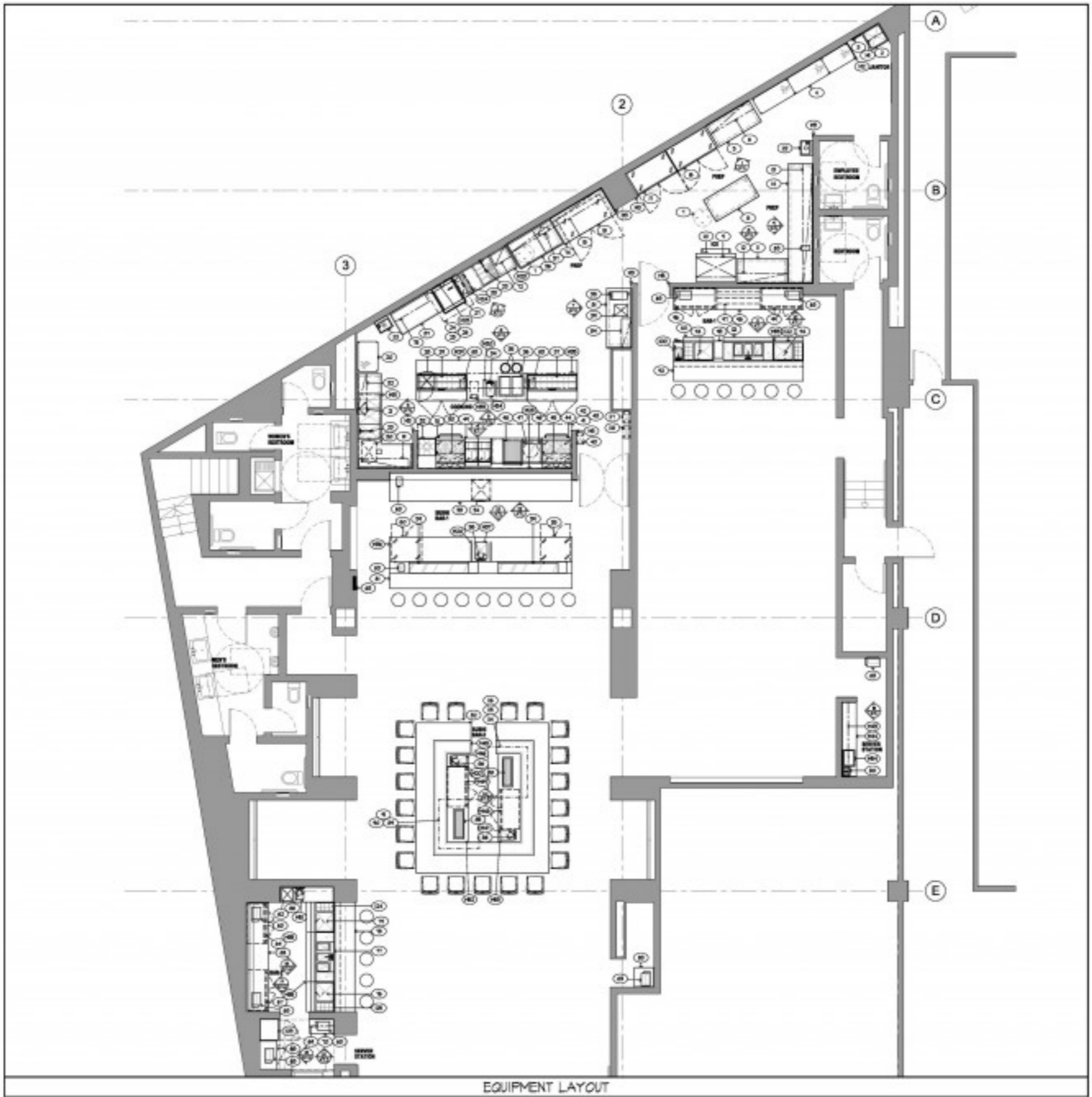
EQUIPMENT LAYOUT
