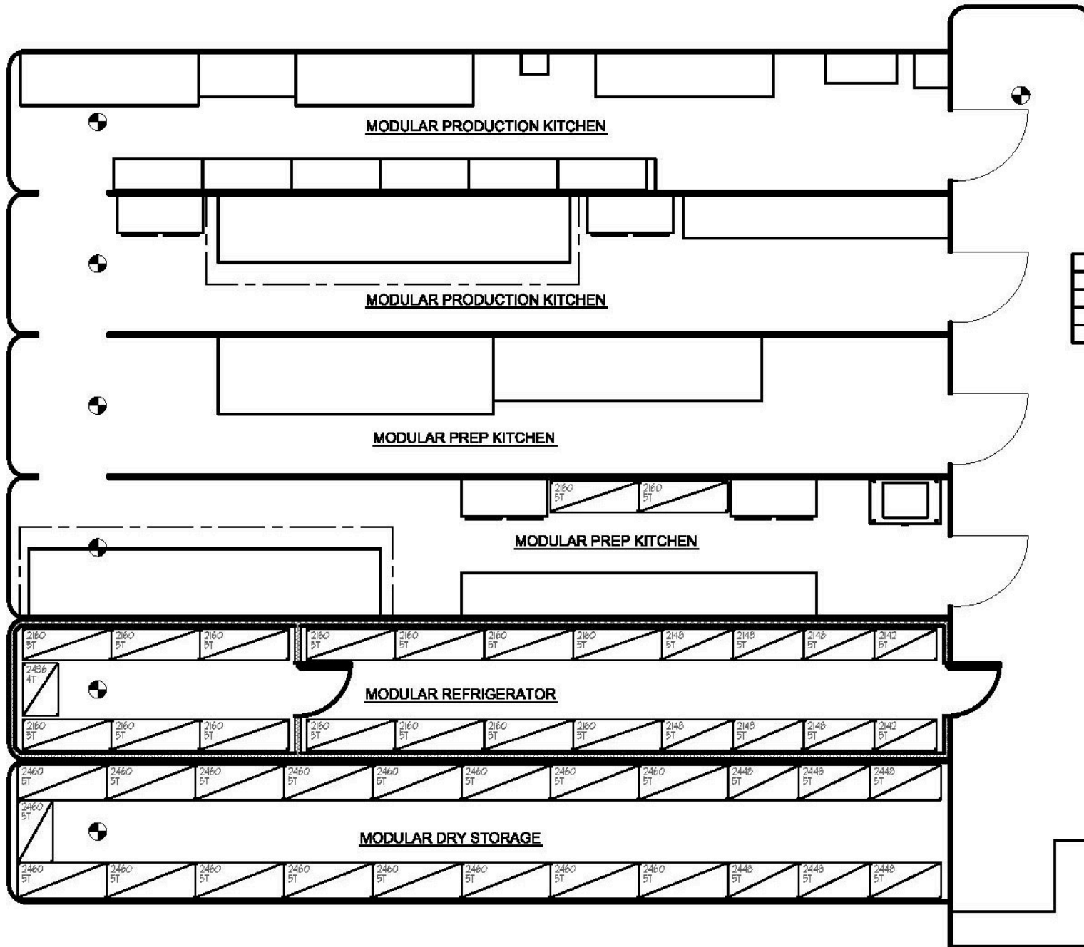
TEMPORARY KITCHENS 123 MODULAR KITCHEN CAPABLE OF 5,000 MEALS PER DAY
